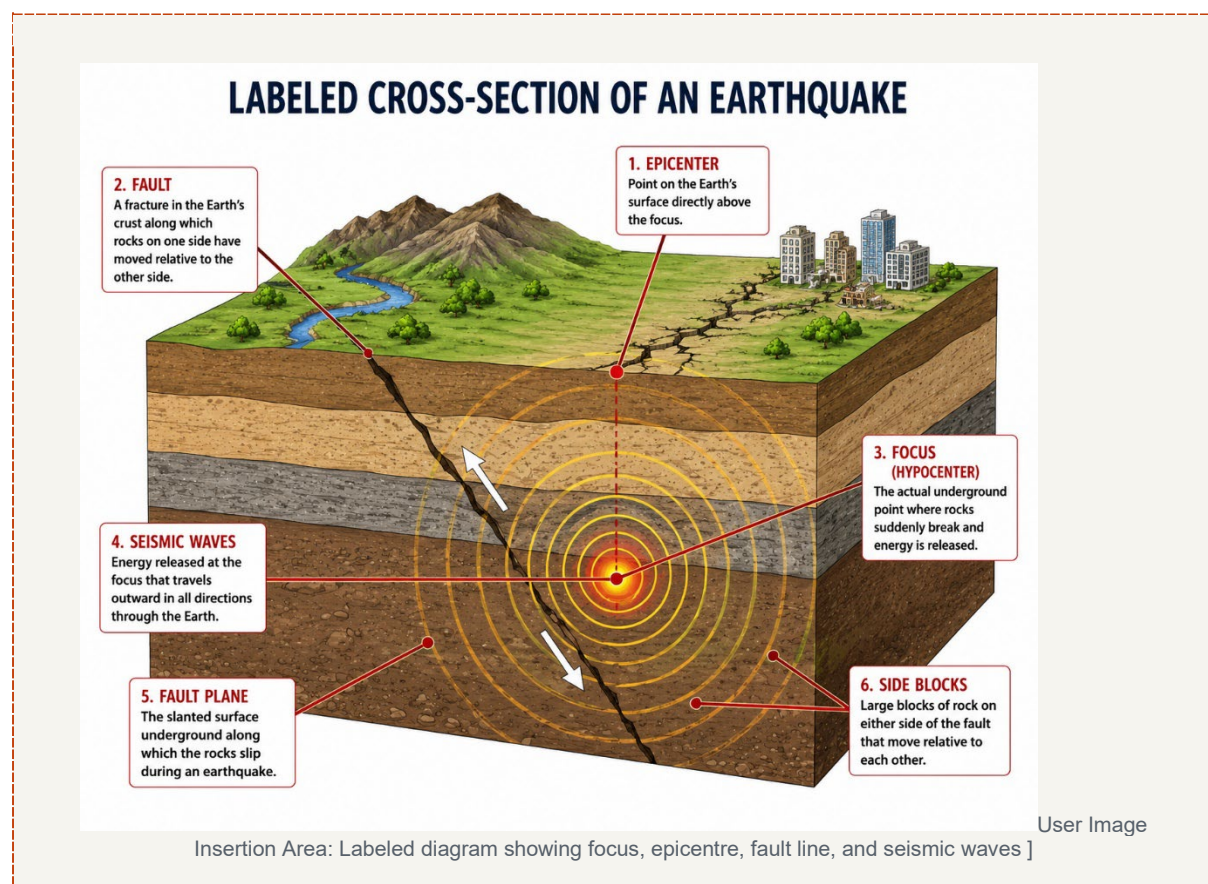
Figure 1 - Earthquake Cross-Section: A cross-sectional view of an active earthquake zone, highlighting the focal point underground, the surface epicentre, and the propagating circular energy waves.
